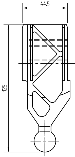
WKS 50 KÜRESEL MAFSAL
