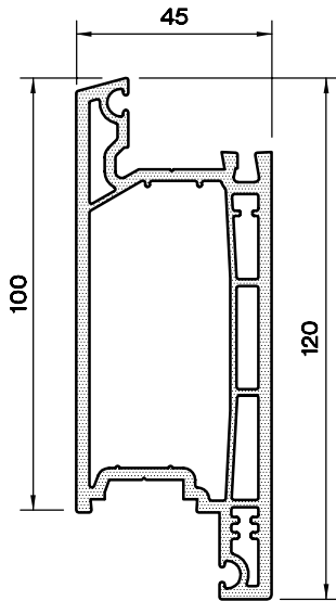
KAPI-100 PROFİLİ 1145.510
