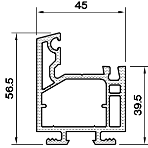
KASA-56 PROFİLİ 1145.156
