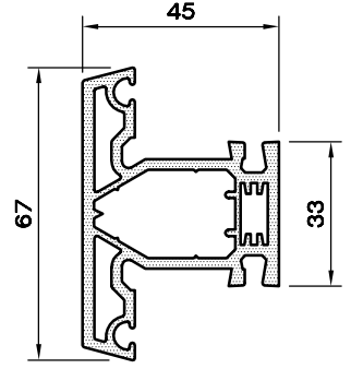
ORTAKAYIT-67 PROFİLİ 1145.367
