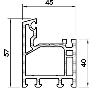
KASA-57 PROFİLİ 1145.157
