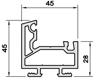
BANYO KASA-45 PROFİLİ 1145.145
