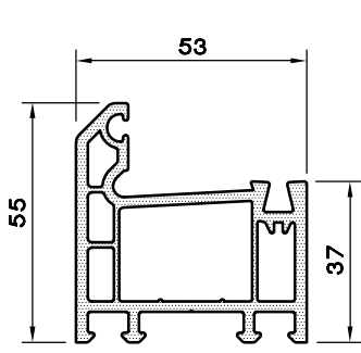
KASA-55/3 PROFİLİ 1153.155
