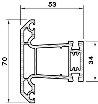
ORTAKAYIT-70/3 PROFİLİ 1153.370
