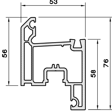
KANAT-56/2 PROFİLİ 1153.256
