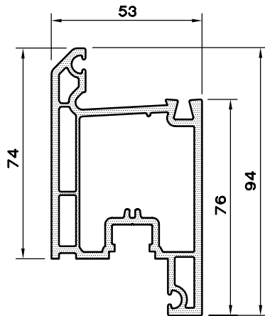
KANAT-74/2 PROFİLİ 1153.474
