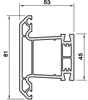
ORTAKAYIT-81/3 PROFİLİ 1153.382
