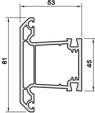
ORTAKAYIT-81/2 PROFİLİ 1153.381
