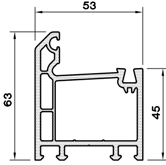
KASA-63/2 PROFİLİ 1153.163
