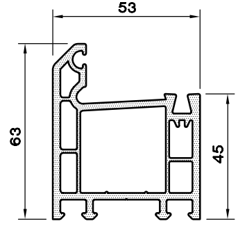
KASA-63/3 PROFİLİ 1153.164
