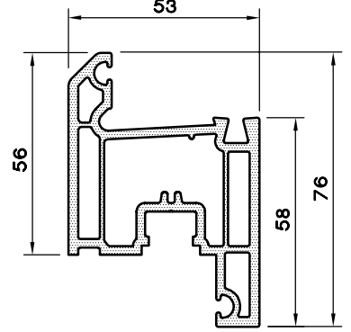
KANAT-56/3 PROFİLİ 1153.257
