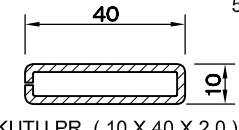
KUTU PR. (10 X 40 X 2.0) 51S7.112
