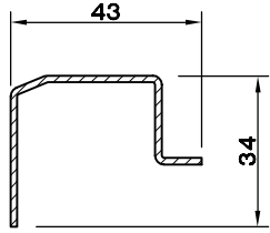
BİNİLİ KANAT -82/2 DESTEK SAÇI (1.5) 5160.231
