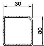
ORTAKAYIT -82 DESTEK SAÇI (30 X 30 X 1.5) 5199.311
