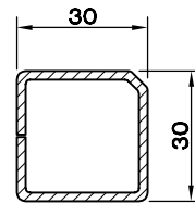
ORTAKAYIT -82 DESTEK SAÇI (30 X 30 X 2.0) 5199.312
