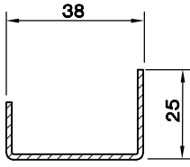
U DESTEK SACI ( 38 X 25 X 1.5 ) 5170.911
