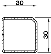
ORTAKAYIT -82 DESTEK SACI ( 30 X 30 X 1.5 ) 5199.311
