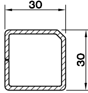
ORTAKAYIT -82 DESTEK SACI ( 30 X 30 X 2.0 ) 5199.312
