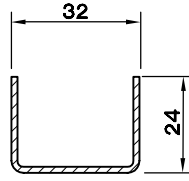
U DESTEK SACI ( 32 X 24 X 1.5 ) 5161.911
