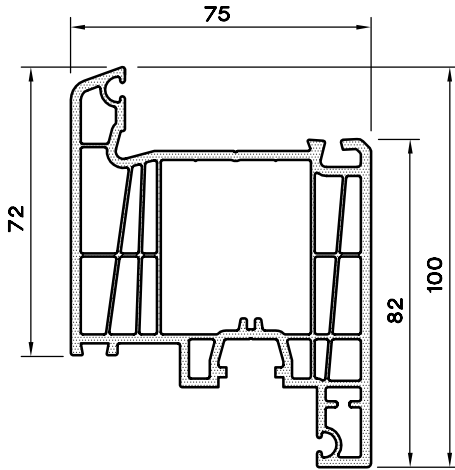
KAPI-72/6 PROFİLİ 1175.572
