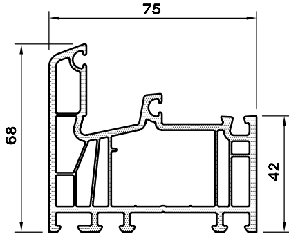
KASA-68/6 PROFİLİ 1175.168
