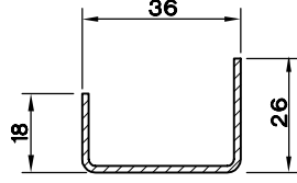
U DESTEK SAÇI 36 X 18 X 26 (1.5) 5175.911
