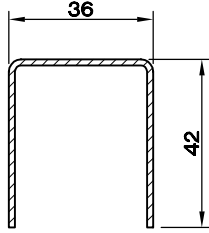
U DESTEK SAÇI 36 X 42 (1.5) 5175.921
