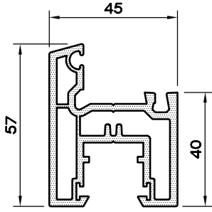
DAR KANAT - 45 PROFİLİ 11S3.245
