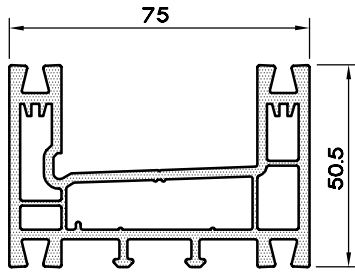
GENİŞ KASA - 75 PROFİLİ 11S1.175
