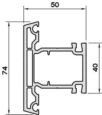
ORTAKAYIT - 74 PROFİLİ 11S1.374
