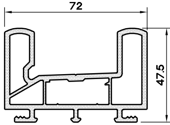
DAR KASA - 72 PROFİLİ 11S3.172
