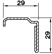
DAR KANAT -45 DESTEK SACI (1.5) 51S2.211
