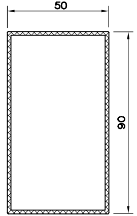
AL. KUTU PR. ( 50 X 90 ) 6099.159
